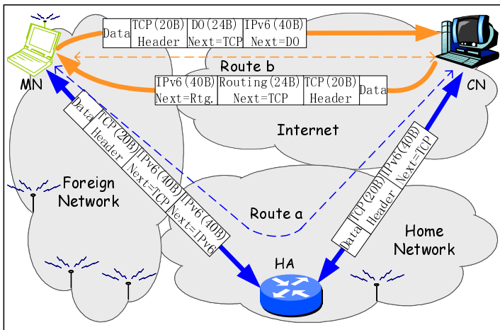
Fig. 1. The mobile packet routing mechanisms in MIPv6
