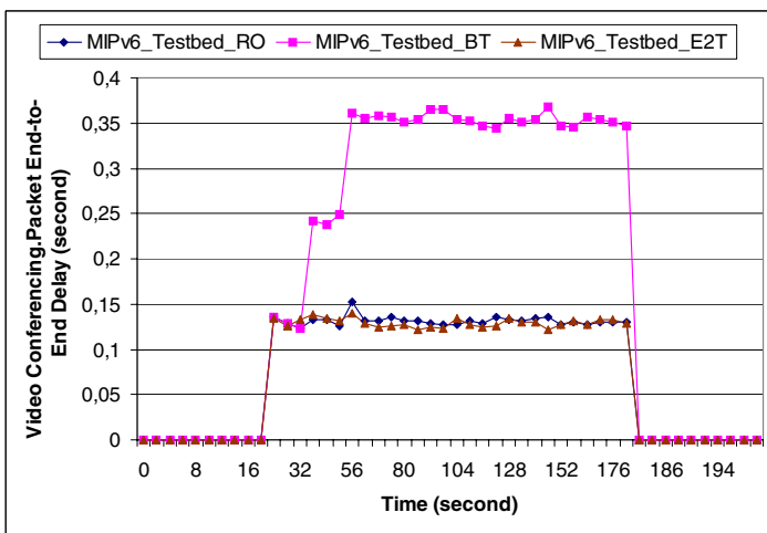
Fig. 6. The end-to-end delays of video conferencing traffic
