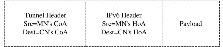
Fig. 3. The IPv6 headers in E 2 T tunneled packets
