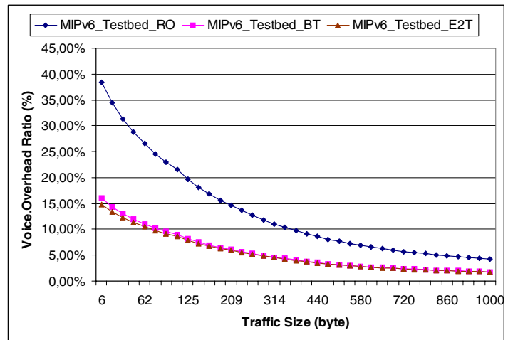
Fig. 5. The overhead ratio in MIPv6
